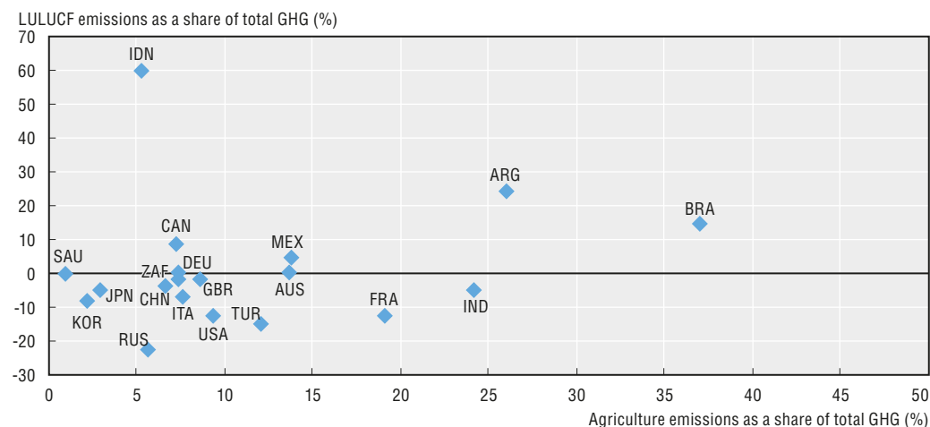
Figure 2.15. G20 agriculture, land-use and forestry emissions as % of total GHG emissions
