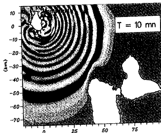
Numerical modelling snapshots of the water surface 10 minutes after a pyroclastic flow on the southeastern part of Monserrat Island led to a submarine landslide and the generation of a tsunami. Courtesy of LDG-France.
