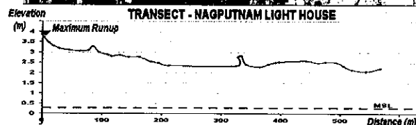
Post-tsunami survey measuring runup along a transect inland from the coast. Courtesy of ICMAM, Chennai, INDIA.
