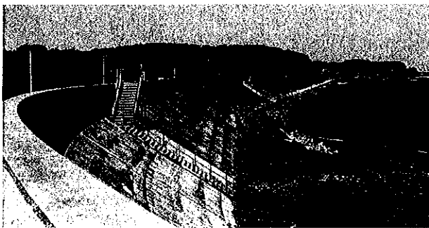
Sea wall with stairway evacuation route used to protect a coastal town against tsunami inundation in Japan. Photo courtesy of River Bureau, Ministry of Land, Infrastructure and Transport, Japan.
