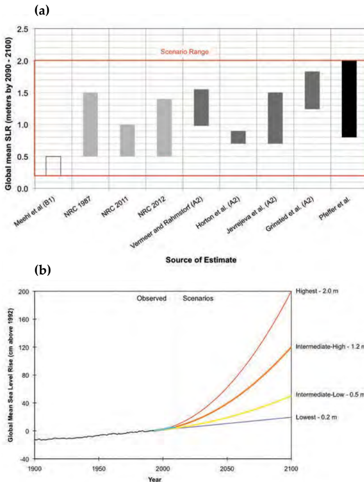
Figure 3-9 (a) End-of-century (~2090–2100) estimates for global mean sea level rise in meters. Meehl et al. (2007) is based on climate model projections for the IPCC and outlined in black. NRC (1987, 2011, and 2012) is based on synthesis of the scientific literature and shown in light gray. Vermeer and Rahmstorf (2009), Horton et al. (2008), Jevrejeva et al. (2010), Grinsted et al. (2009) are based on semi-empirical approaches and shown in dark gray. Pfeffer et al. (2008) is a calculation of the maximum possible contribution from ice sheet loss and glacial melting and shown in black. (b) Global mean sea level rise scenarios developed for the 2013 NCA. Present mean sea level (MSL) for the US coasts is determined from the National Tidal Datum Epoch (NTDE) provided by NOAA. The NTDE is calculated using tide gage observations from 1983–2001 and 1992, the mid-point of the NTDE, is chosen as a starting point. (From Parris et al., in press).
