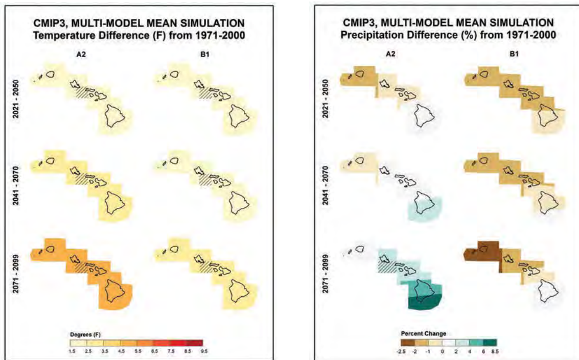
Figure 1-8 Multi-model mean annual differences in (left) temperature (°F) and (right) precipitation (%) in Hawai'i between the three future periods and 1971–2000, from the 15 CMIP3 model simulations. (Courtesy of Ken Kunkel, NOAA NCDC and North Carolina State University.)
