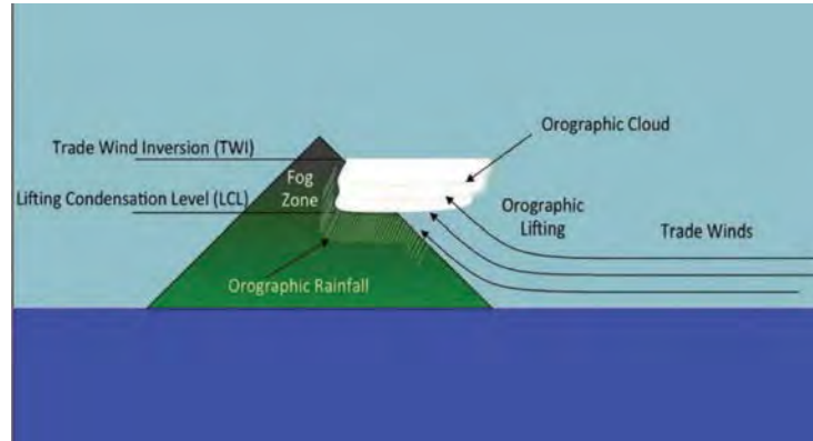
Figure 2-2 Depiction of the orographic effect. The amount and location of rainfall in Hawai'i and other high islands is strongly controlled by orographic processes. As warm air approaches a mountain range, it rises, cools, and condenses in orographic clouds, causing rainfall. On very high mountains in Hawai'i, as the cooled air continues to rise, it reaches the trade wind inversion layer, at which point the air again warms, and above which there is little to no precipitation. (From Giambelluca et al., 2011.)
